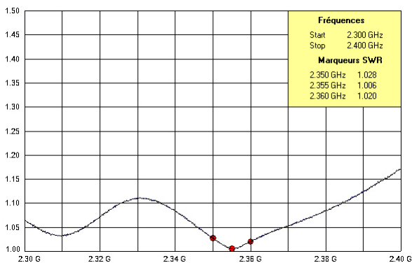
VSWR CURVE
