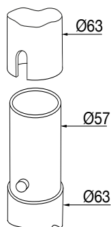
MTLV interface
