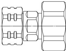
4.3-10 m / 7-16 m
