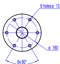
antenna fixing
