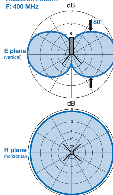
Radiation Pattern F: 400 MHz
